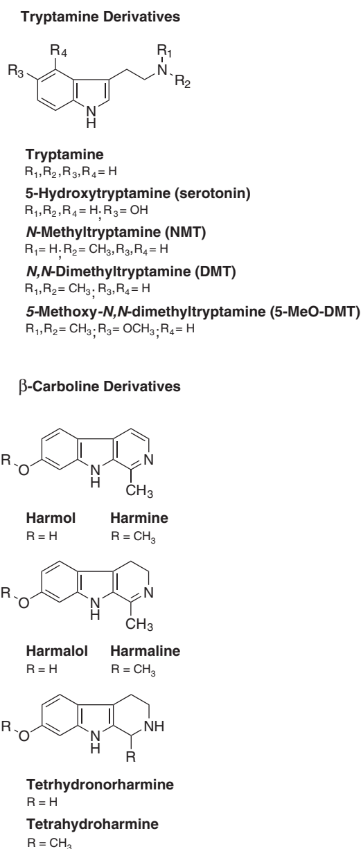
Figure 1. General chemical structure of the tryptamine and β-carboline derivatives.
